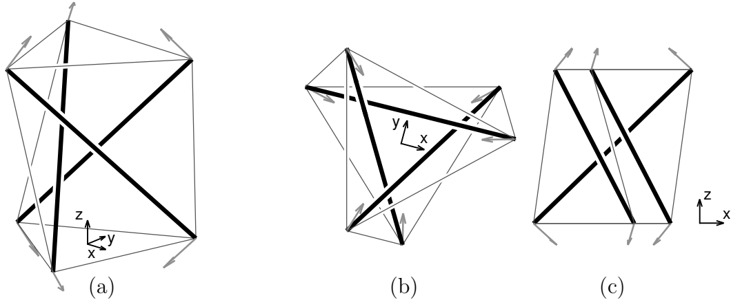
Fig. 6. Fully symmetric zero-stiffness mode, with (a) 3D view, (b) top view and (c) side view. All displacement vectors are of equal magnitude, and with equal z-component. In this mode the rotation angle between bottom and top triangle remains constant throughout the displacement.
