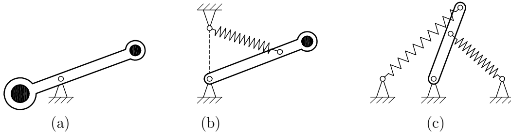
Fig. 1. Static balancing: the three structures shown are in equilibrium for any position of the bar, as long as in (a) the masses (black circles) are correctly chosen, and in (b) and (c) the springs are zero-free-length springs with appropriately chosen stiffness.
